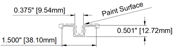
ALUMABOARD JOINT TOP REVEAL
