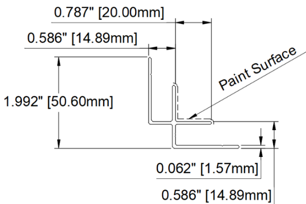
ALUMABOARD INSIDE CORNER
