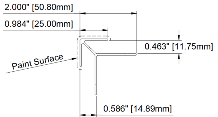
ALUMABOARD OUTSIDE CORNER
