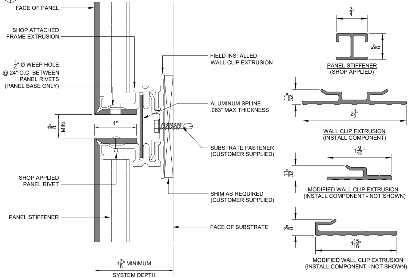
ALUMINUM PLATE SERIES "AP400" RAINSCREEN SYSTEM (SECTION A - HORIZONTAL & VERTICAL PANEL JOINT)
