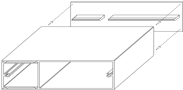
2"X8" Batten Assembly
