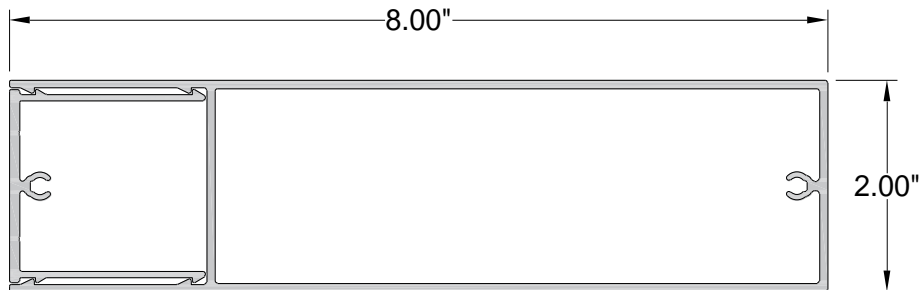
2" X 8" Batten Assembly
