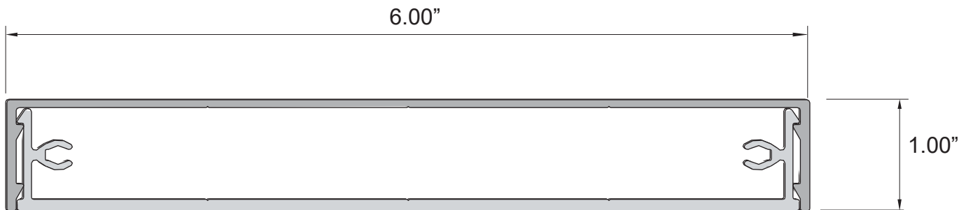
1"x 6" Horizontal Interlocking Batten
