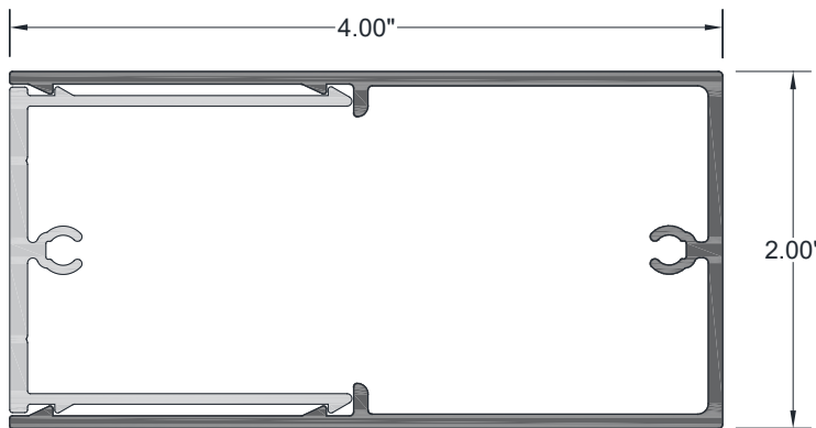
2" X 4" Vertical Interlocking Batten
