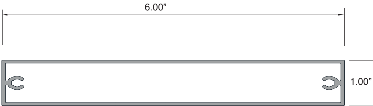
1" x 6" Batten #1.18 LBS/lnft
