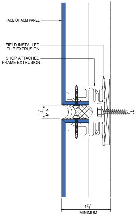
ACM Series A2000 Wet System
