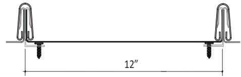
PS-10 Batten Seam Panel
