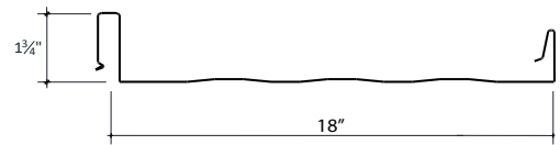
SL-175 Snap Lock Panel
