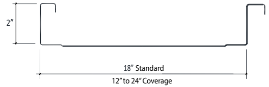
MS-200 Mechanical Lock Standing Seam Panel
