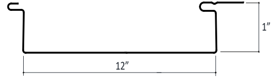
FW-10 Flush Wall Panel
