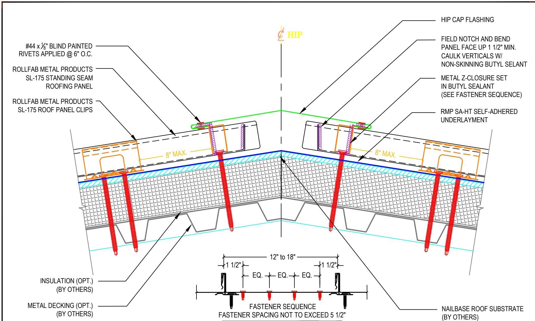
ANCHORING FASTENER PATTERN
