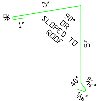
HIGH EAVE / PEAK FLASHING (HE1)
