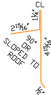
HIGH EAVE / PEAK CLEAT (HE1CL)
