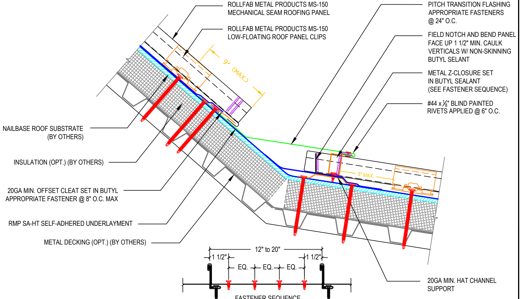
FASTENER SEQUENCE FASTENER SPACING NOT TO EXCEED 5 1/2" ANCHORING FASTENER PATTERN
