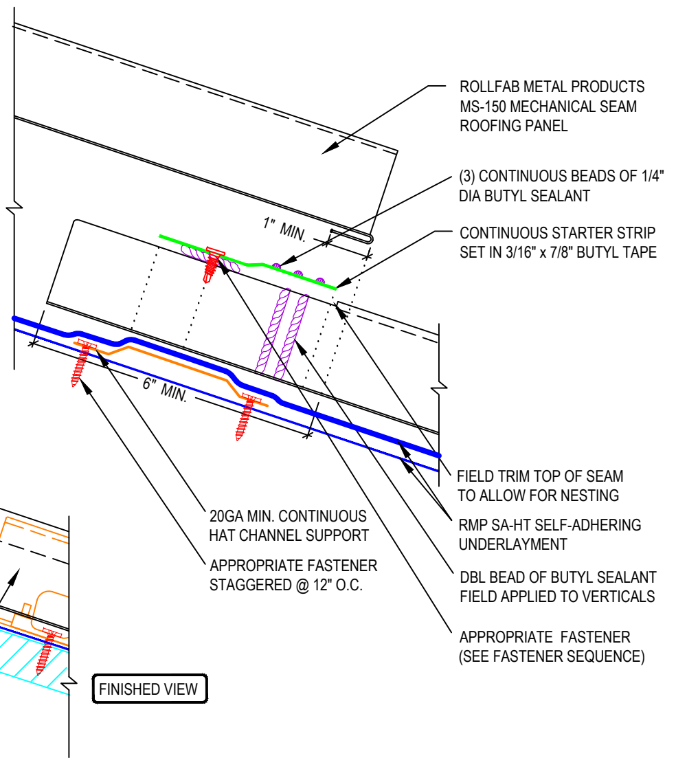
EXPLODED VIEW
