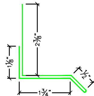
DRIP FLASHING
