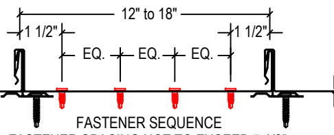
FASTENER SEQUENCE FASTENER SPACING NOT TO EXCEED 5 1/2" ANCHORING FASTENER PATTERN
