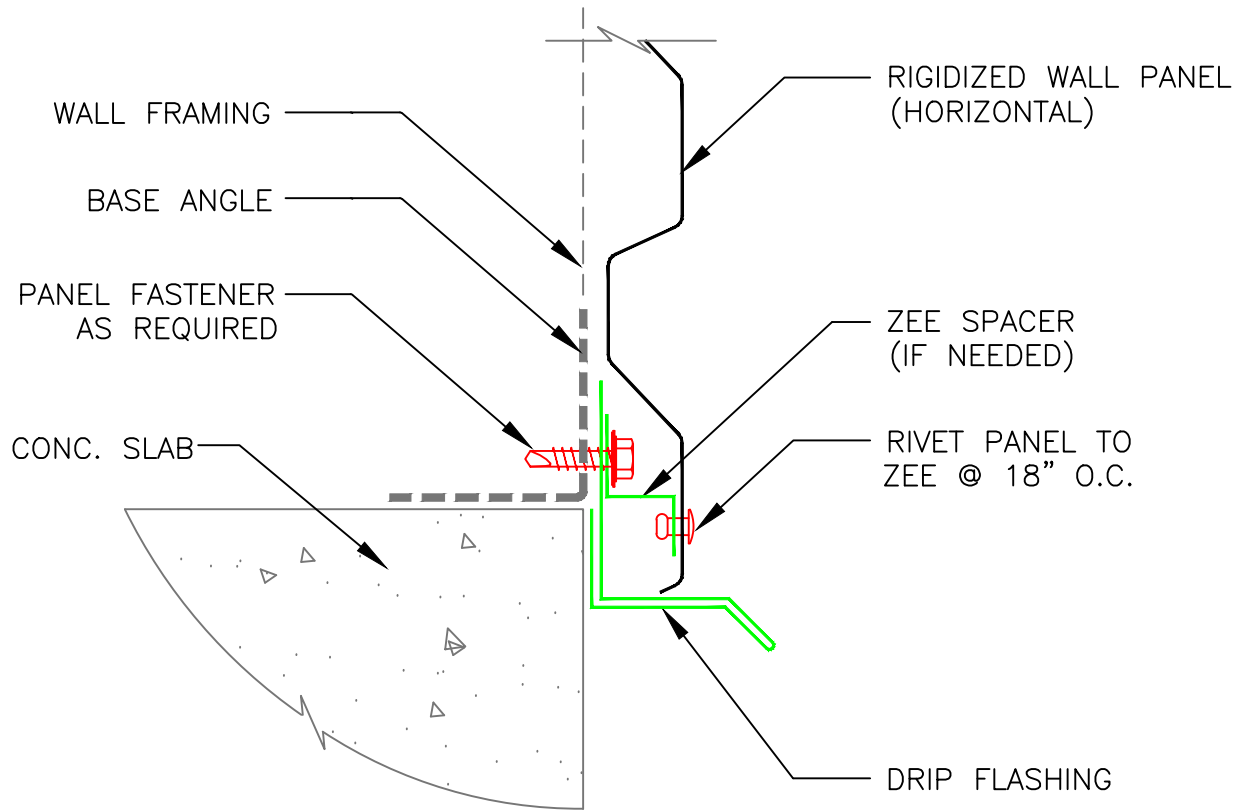
RIGIDIZED WALL PANEL PROFILE
