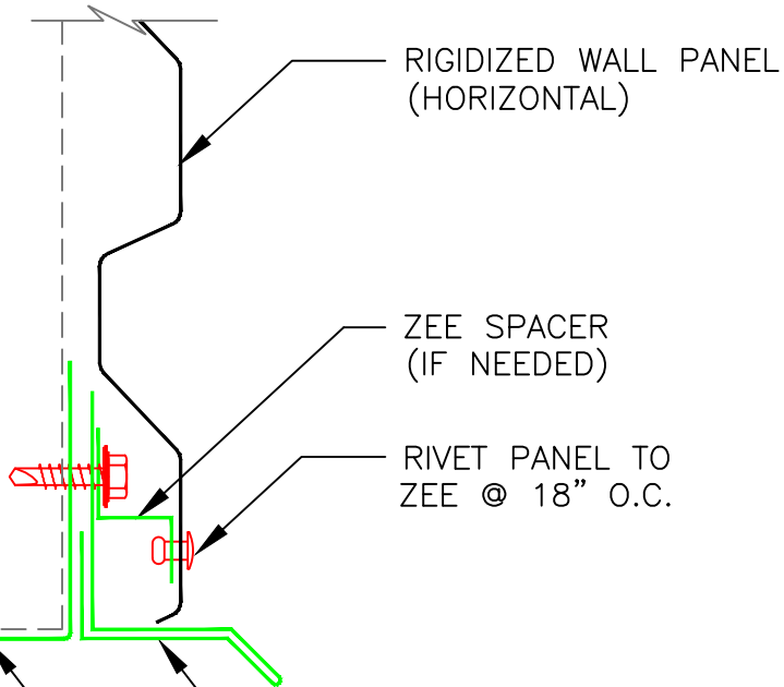
DRIP FLASHING
