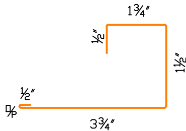
BOX RAKEWALL CLEAT (BRW/C1)
