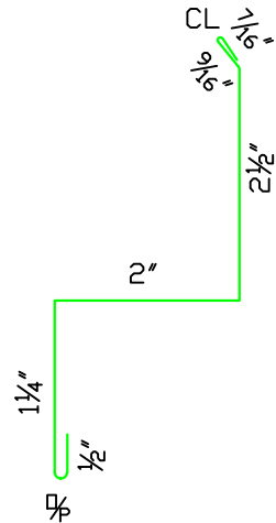
BOX RAKEWALL FLASHING (BRW1)
