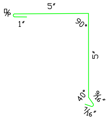
RAKE / GABLE FLASHING (RGZ1)
