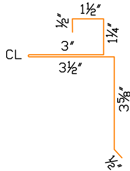
RAKE / GABLE CLEAT (RGZC1)
