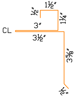
BOX RAKE / GABLE CLEAT (BRG/C1)
