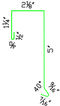
BOX RAKE / GABLE FLASHING (BRG1)
