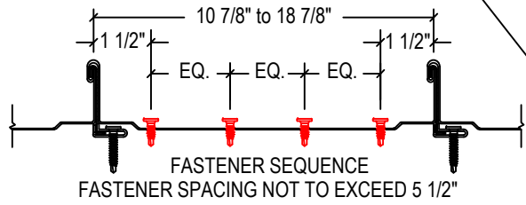
FASTENER SEQUENCE FASTENER SPACING NOT TO EXCEED 5 1/2" ANCHORING FASTENER PATTERN
