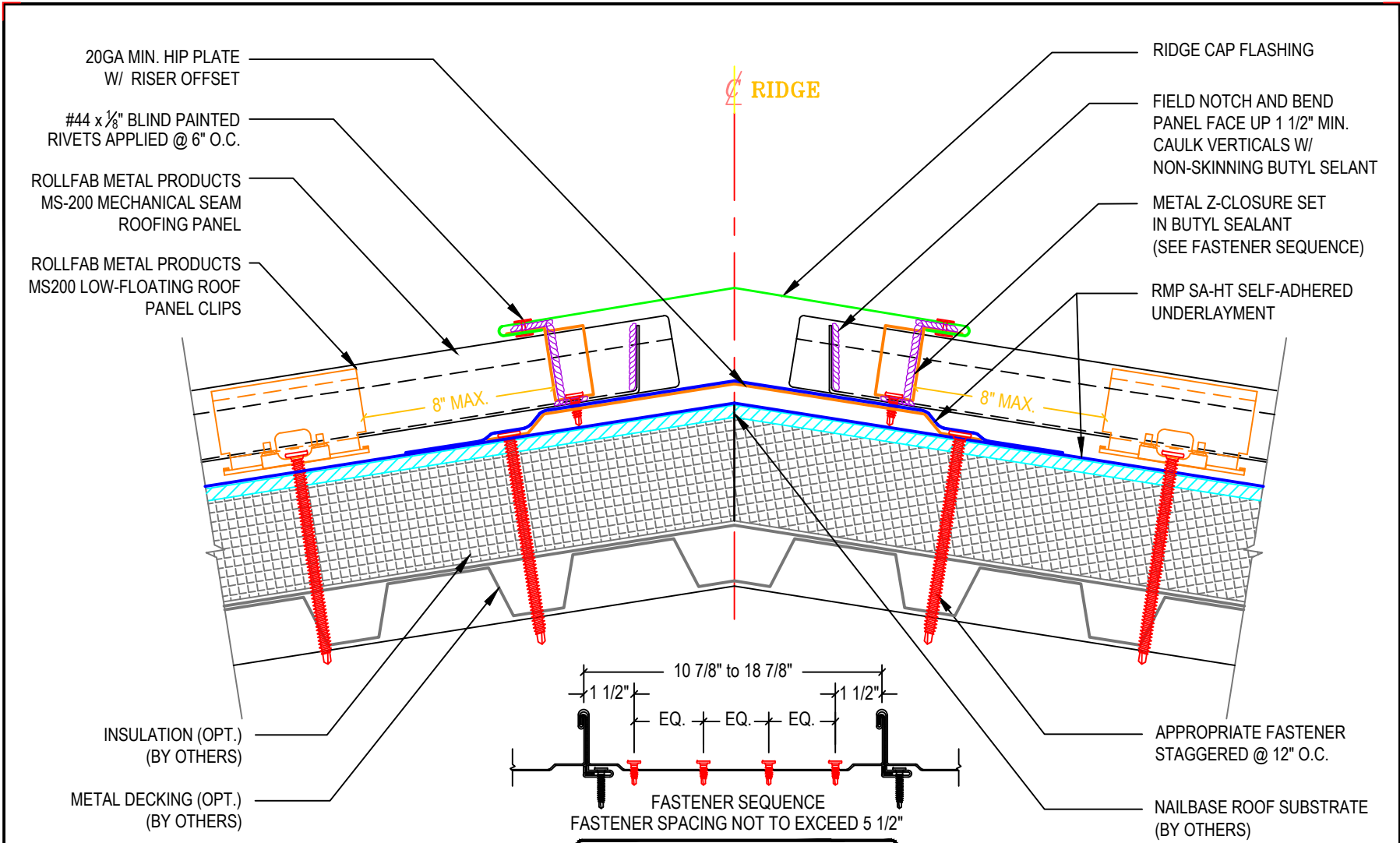
FASTENER SEQUENCE FASTENER SPACING NOT TO EXCEED 5 1/2" ANCHORING FASTENER PATTERN
