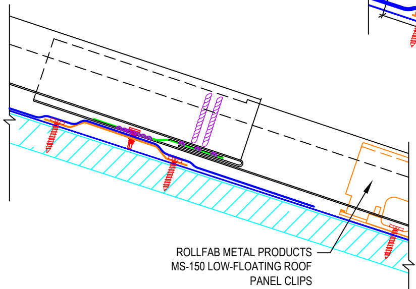
EXPLODED VIEW
