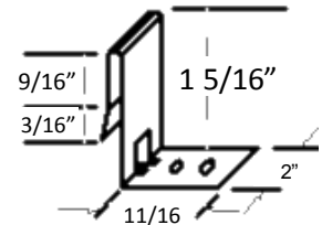
Clip Diagram
